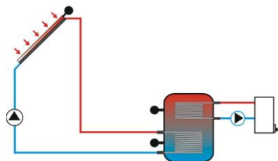
Heat tank to constant temperature
